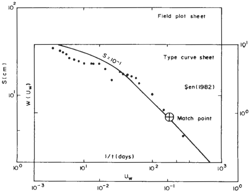
FIG. 6. Pumping test in upstream.
